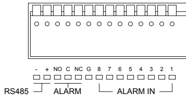
[Fig. 5-6 SENSOR IN PIN]
